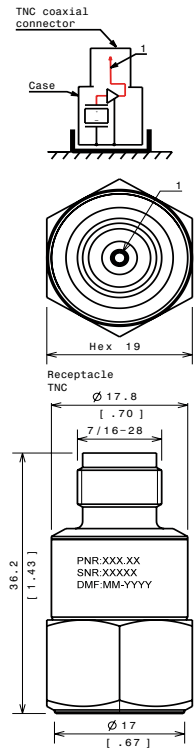
fig 1b : Outline drawing & Electrical layout, B=2 (M12 glass seal)
